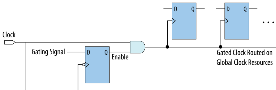
Figure 13. Recommended Clock-Gating Technique for Clock Active on Rising Edge
