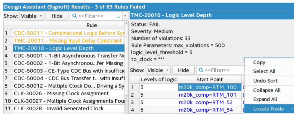
Figure 34. Locate in RTL Viewer
